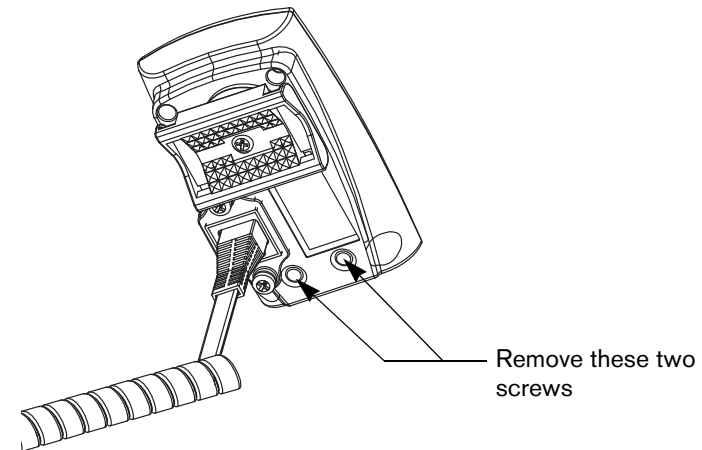
Figure 3: Remove screws holding headphone jack
